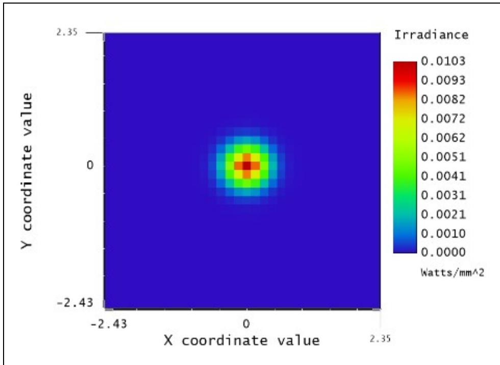
Figure 31: Cylindrical Lens Profile X Dimension
