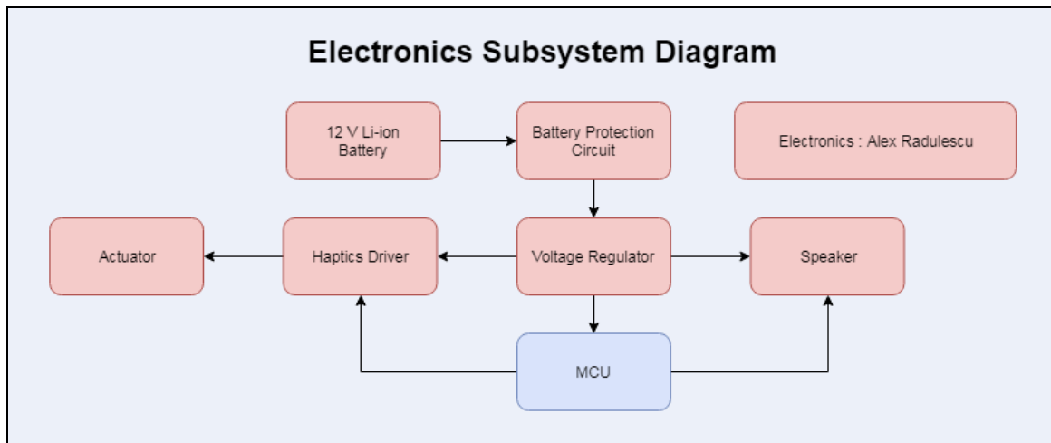
Figure 46: Electronics Block Diagram (Permission not needed)
