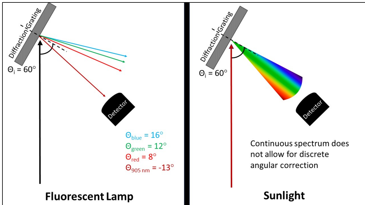
Figure 37: Diffraction Gratings {Kasap, 2013 #22}
