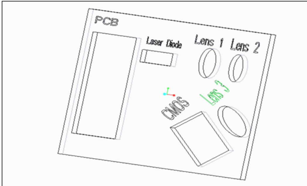
Figure 60: Front Side View of Optical Housing (Permission not needed)
