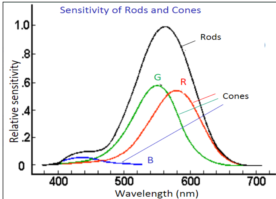
Figure 42: Eye Sensitivity Spectrum (Permission Requested)
