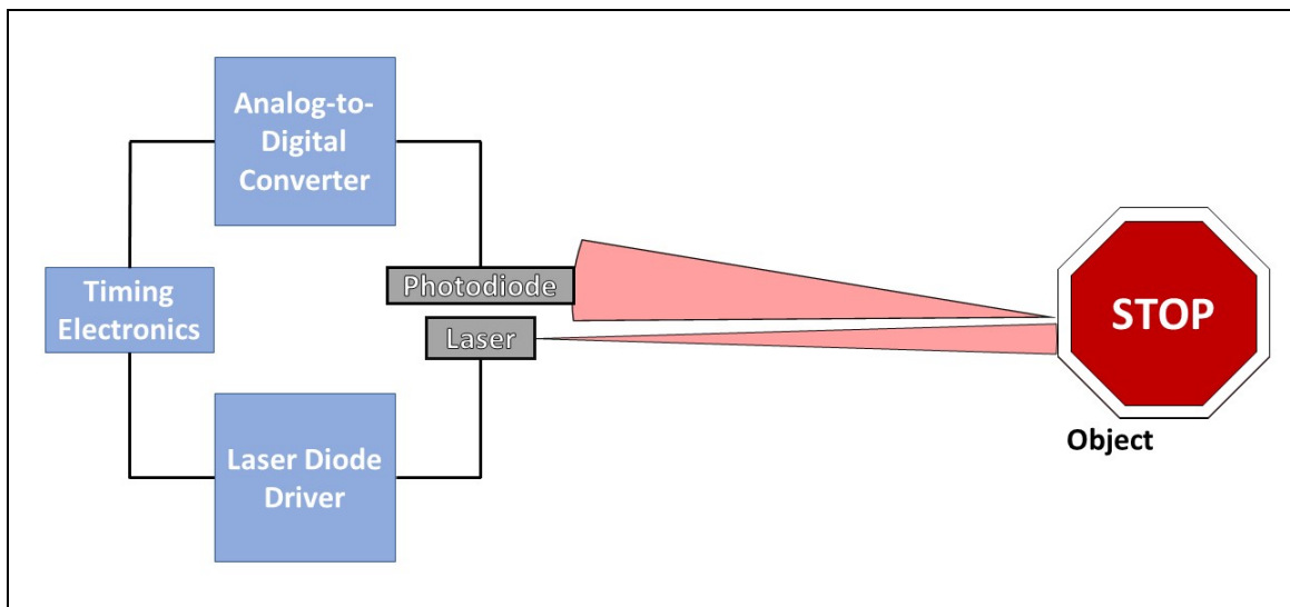
Figure 50: LIDAR (Electronic t_0 ) System Diagram (Permission not needed)
