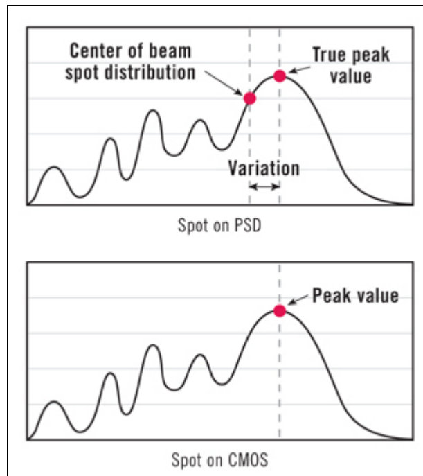
Figure 22: Detector Responsivity (Permission requested) {mtiinstruments, 2018 #23}
