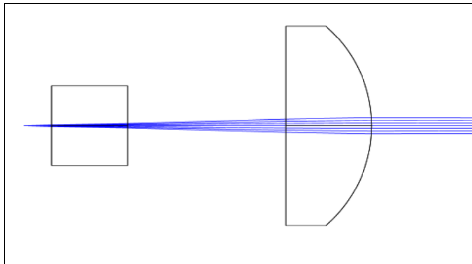
Figure 25: Collimation using Two Plano-Convex Cylindrical Lenses Y View (No Permission Needed)
