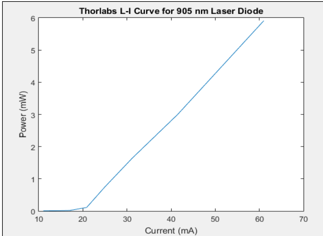
Figure 63: Current-Output Power for Thorlabs L904P010 905 nm Near Infrared Laser Diode (No Permission Needed)
