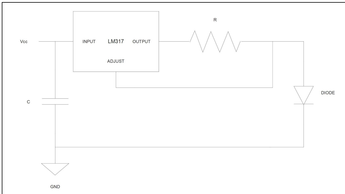
Figure 49: LM317 Constant Current Laser Diode Driver Schematic (No permission needed)
