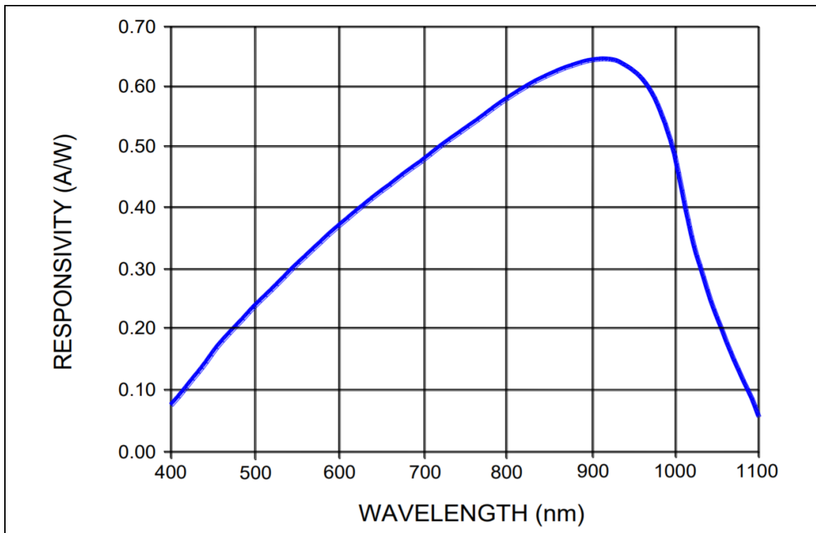
Figure 21: Wavelength vs Responsivity (Permission requested)
