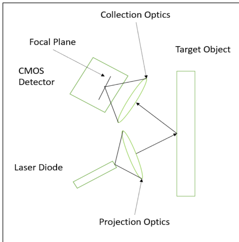
Figure 55: Regular Reflection Model (Permission not needed)
