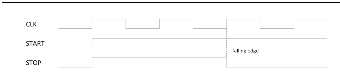
Figure 56: Falling edge clock detection
