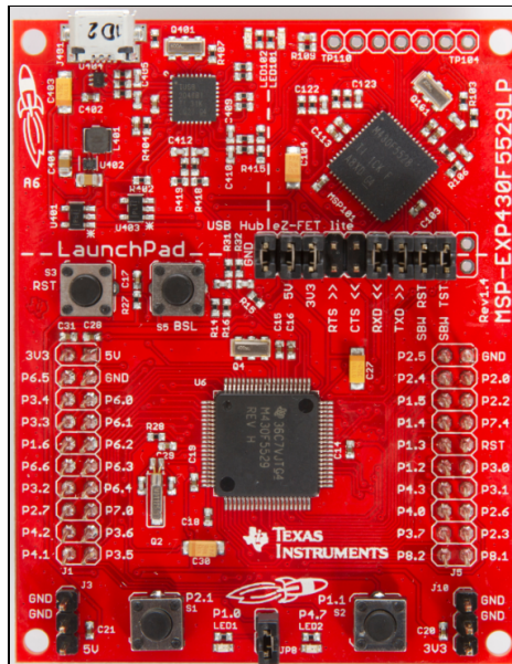
Figure 40: MSP430F5529 LaunchPad (Permission requested)
