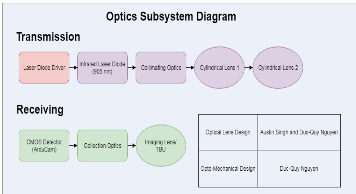
Figure 45: Optics Flow Block Diagram (Permission not needed)
