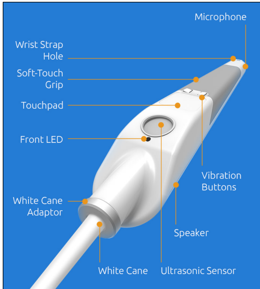
Figure 4: WeWalk Features (Permission requested)
