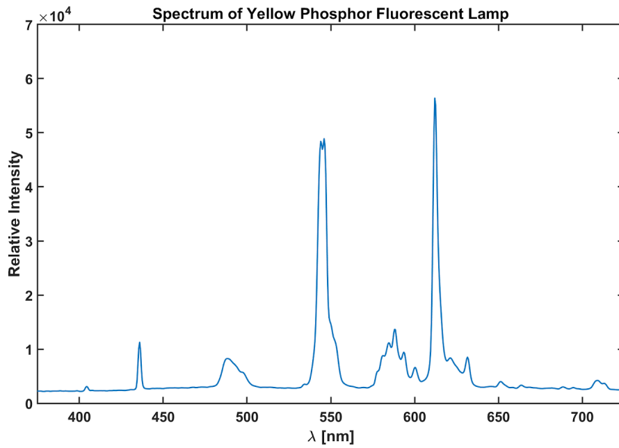
Figure 34: Spectrum of Yellow Phosphor Fluorescent Lamp (No permission needed)
