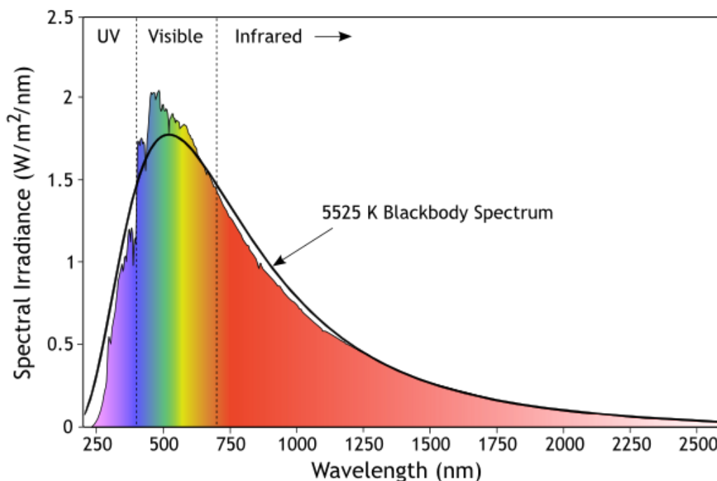
Figure 36: Solar Spectrum (Permission requested) {Kasap, 2013 #22}
