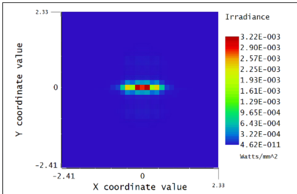
Figure 29: Physical Optics Propagation #2 (No Permission Needed)
