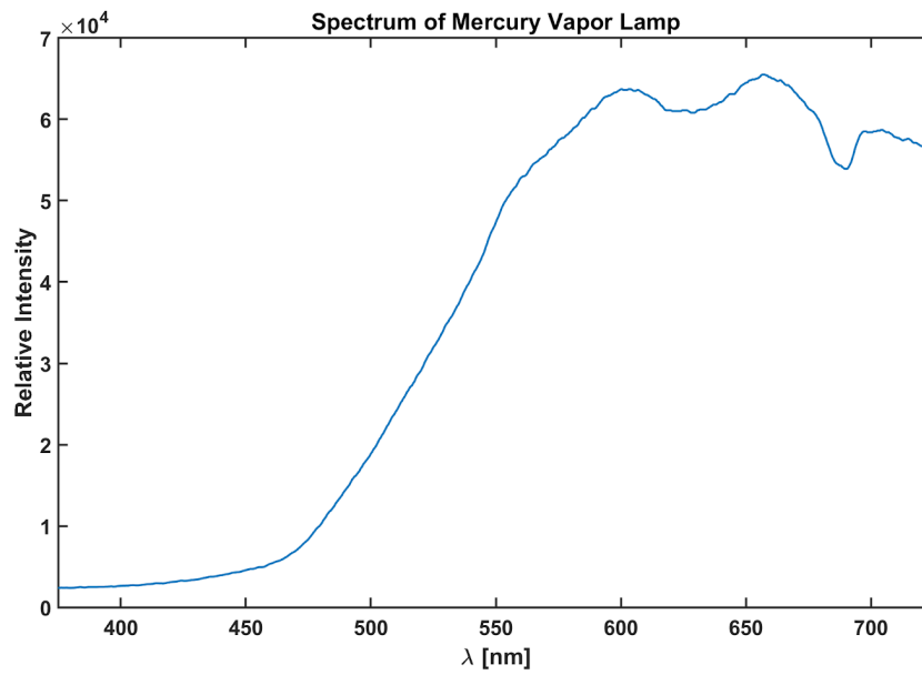
Figure 35: Spectrum of Mercury Vapor Lamp (No permission needed)
