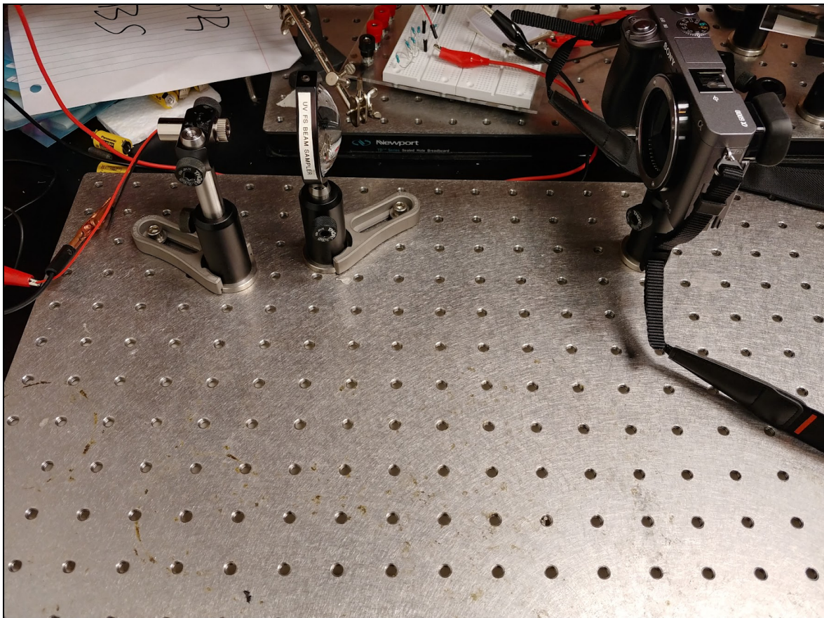
Figure 64: Optical Alignment for Collimation using Single Spherical Lens
