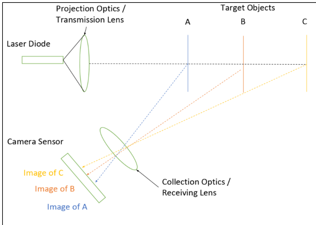
Figure 54: Specular Reflection Method (Permission not needed)
