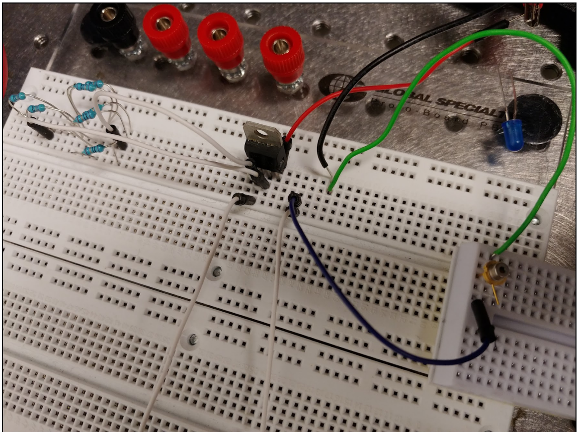
Figure 62: Breadboard Testing of Laser Diode Driver
