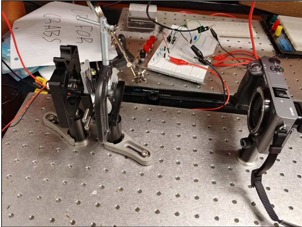
Figure 66: Optical Alignment for Collimation using Two Plano-Convex Cylindrical Lenses (No Permission Needed)
