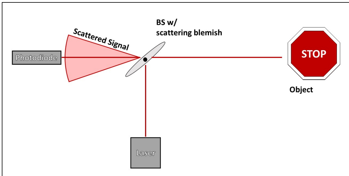
Figure 51: LIDAR (Optical t_0 ) System Diagram (Permission not needed)
