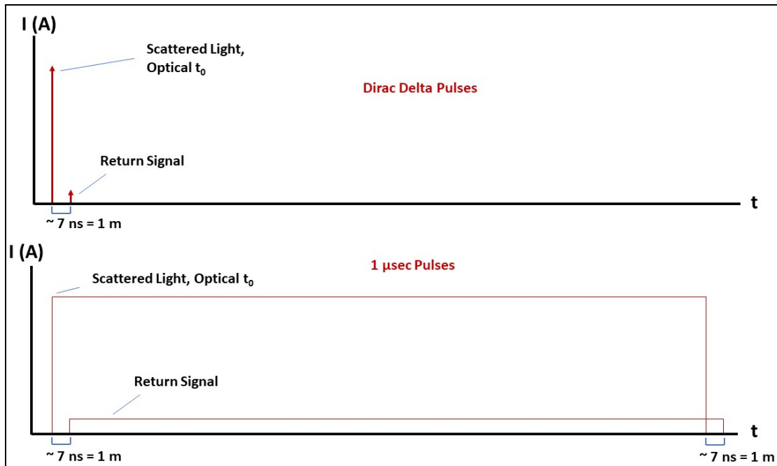
Figure 52: Optical t_0 Signal Pulses (Permission not needed)
