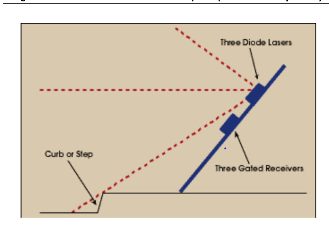
Figure 7: LaserCane™ Detection Description (Permission requested)
