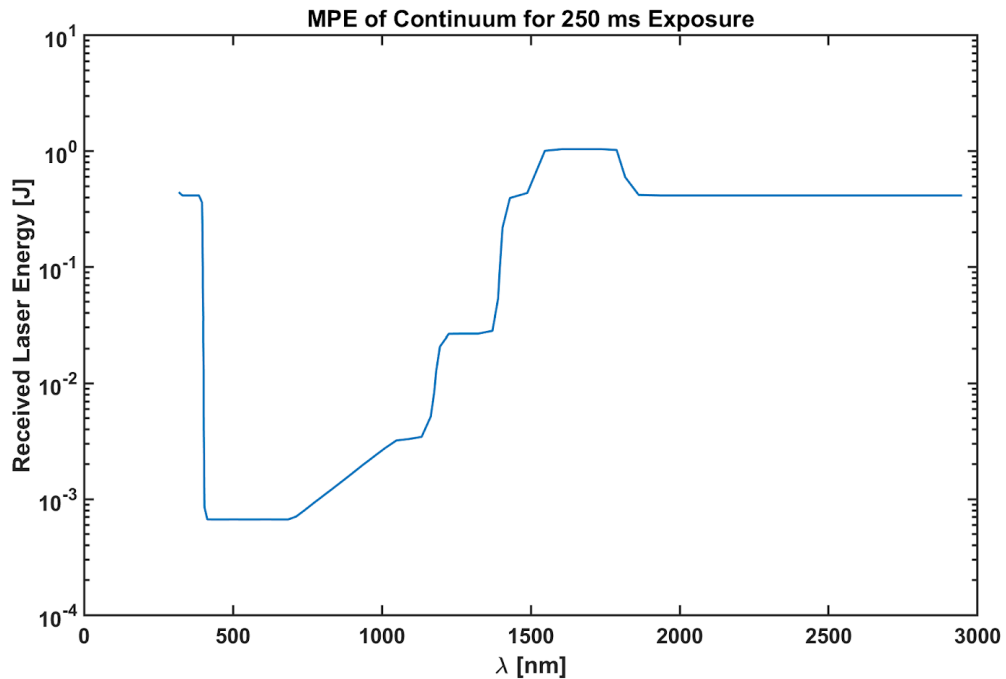
Figure 47: 250 ms Exposure Energy Graph (No permission needed)
