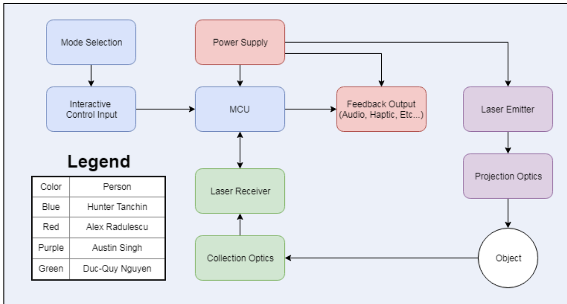
Figure 43 : System Block Diagram (Permission not needed)
