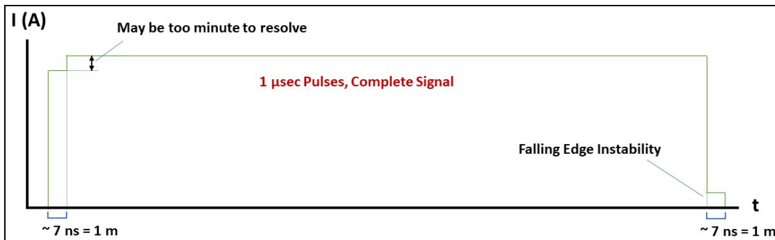
Figure 53: Optical t_0 Signal Concerns (Permission not needed)
