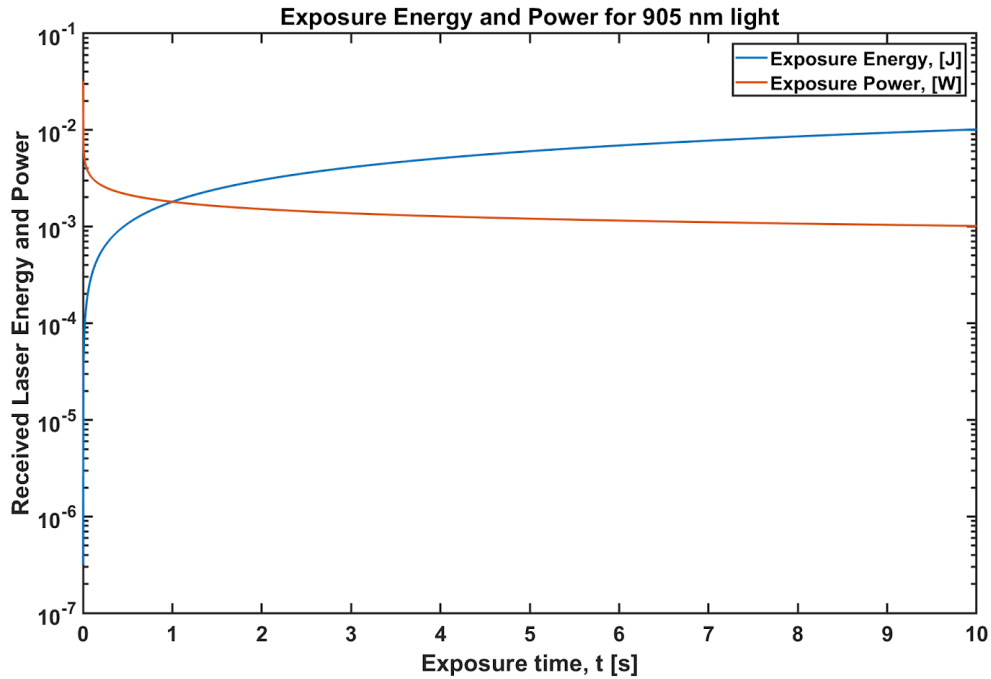
Figure 48: Laser Exposure Energy and Power (No permission needed)
