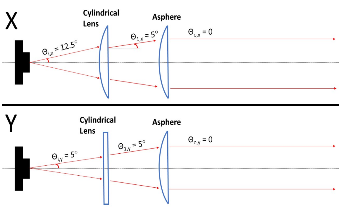
Figure 23: Collimation of Laser Beam using Cylindrical Lens and Asphere (No permission needed)
