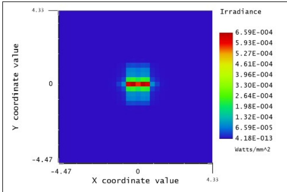
Figure 33: Cylindrical Lens Profile Y Dimension
