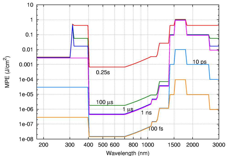
Figure : 41 MPE Vs Wavelength (Permission Requested)
