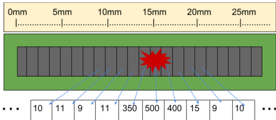
Figure 58: Linear Image Sensor Array Value Storage and Measurement (No permission needed)
