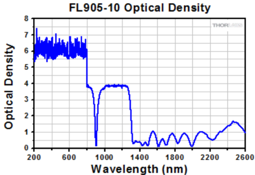
Figure 68: Optical Bandpass Filter (Permission requested)
